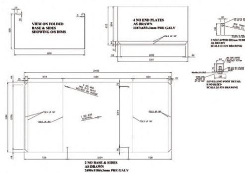
Above left / Metal fabrication detail of the planter
