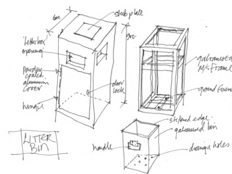
Sketch design of the litter bin
