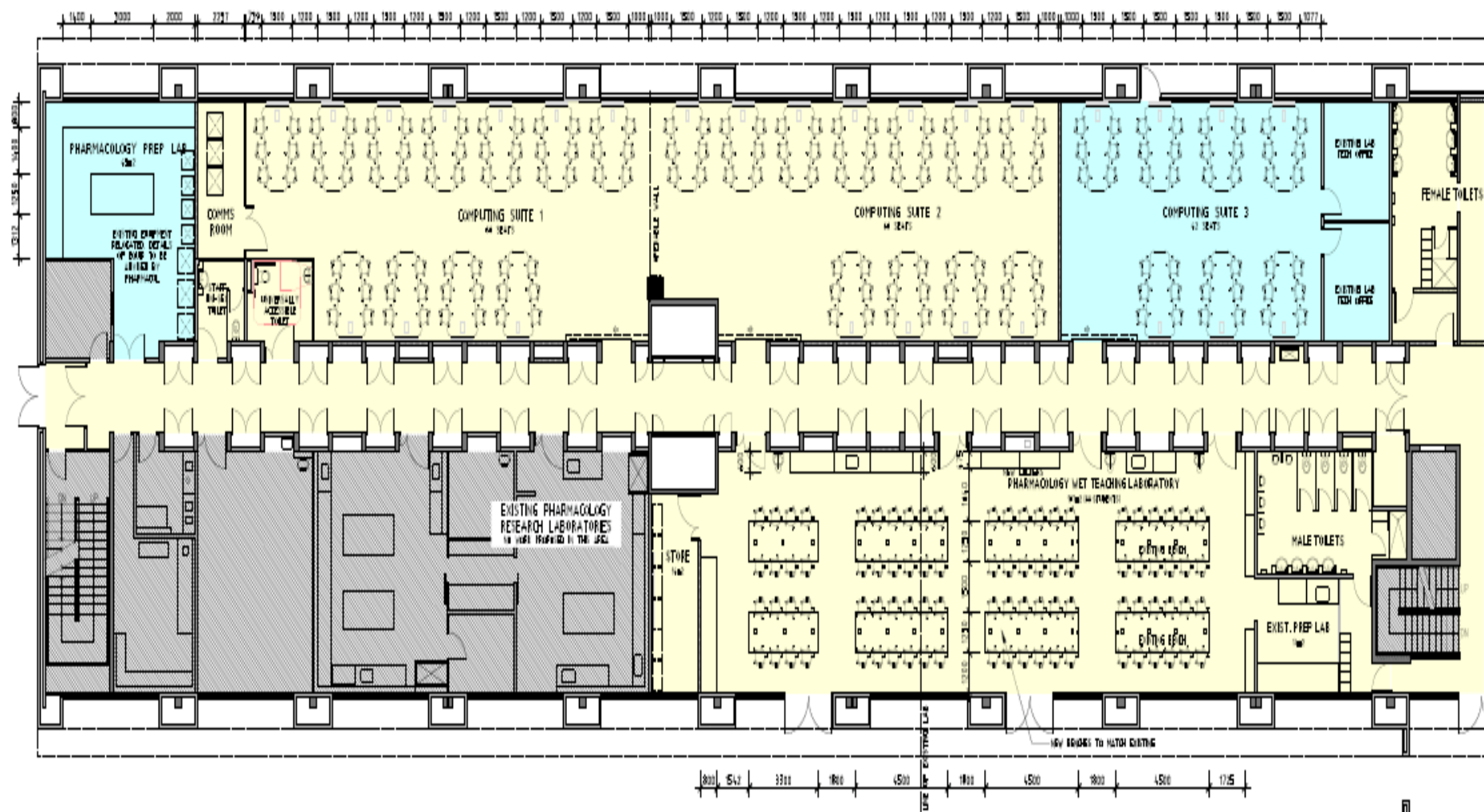
M BLOCK - GROUND FLOOR PLAN WEST WING SCALE 1:100
